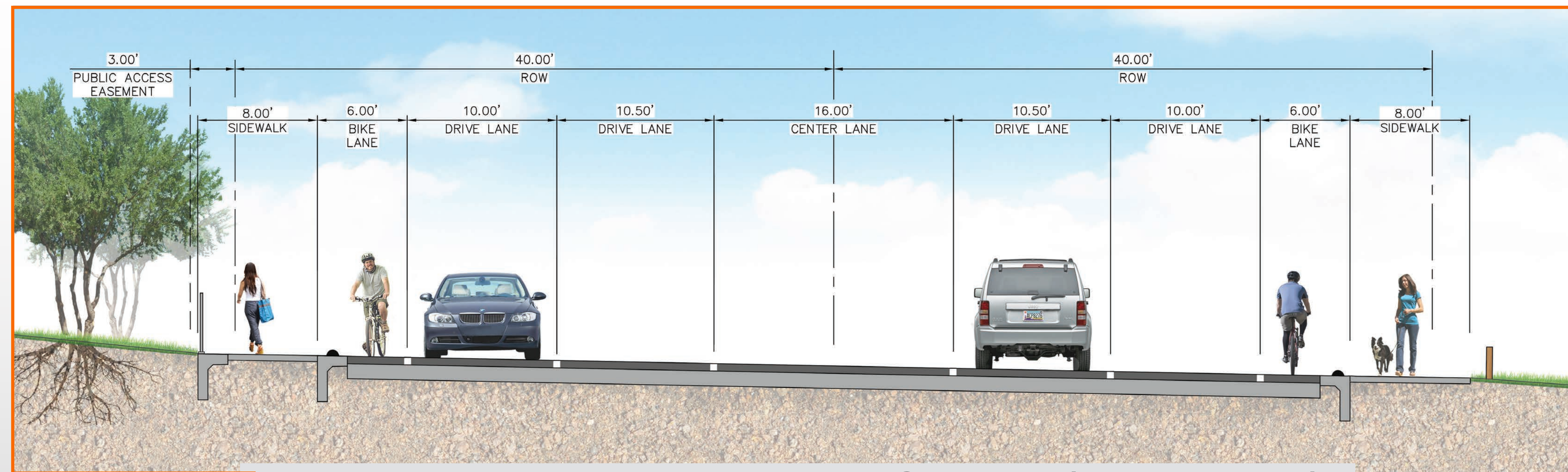
Osborn Road at Indian Bend Wash Crossing (Looking East)
