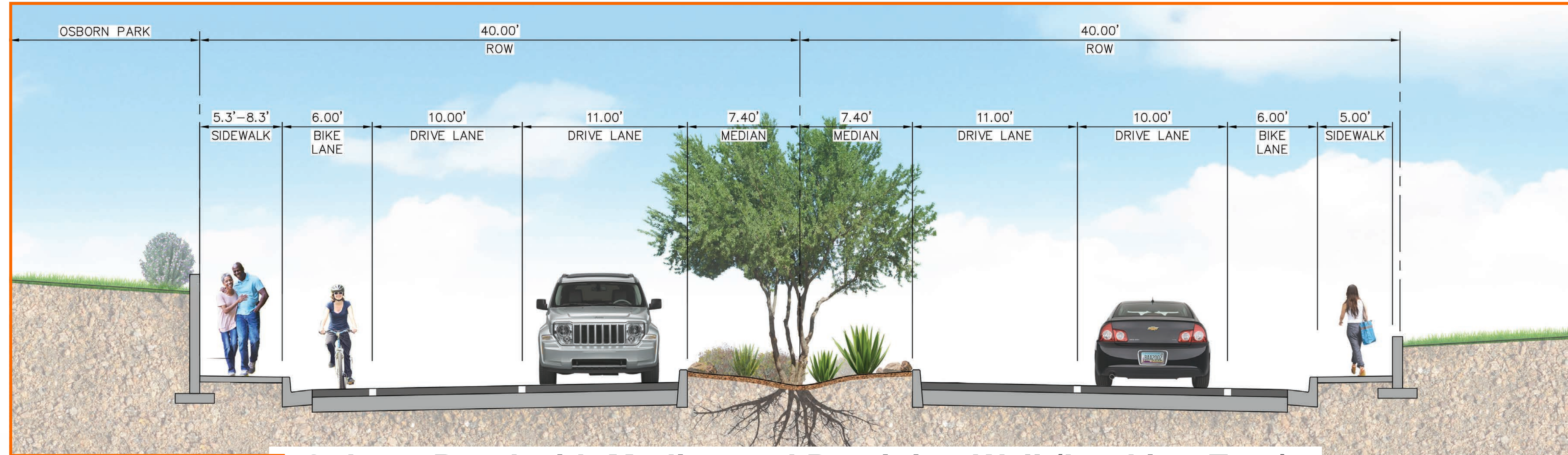
Osborn Road with Median and Retaining Wall (Looking East)
