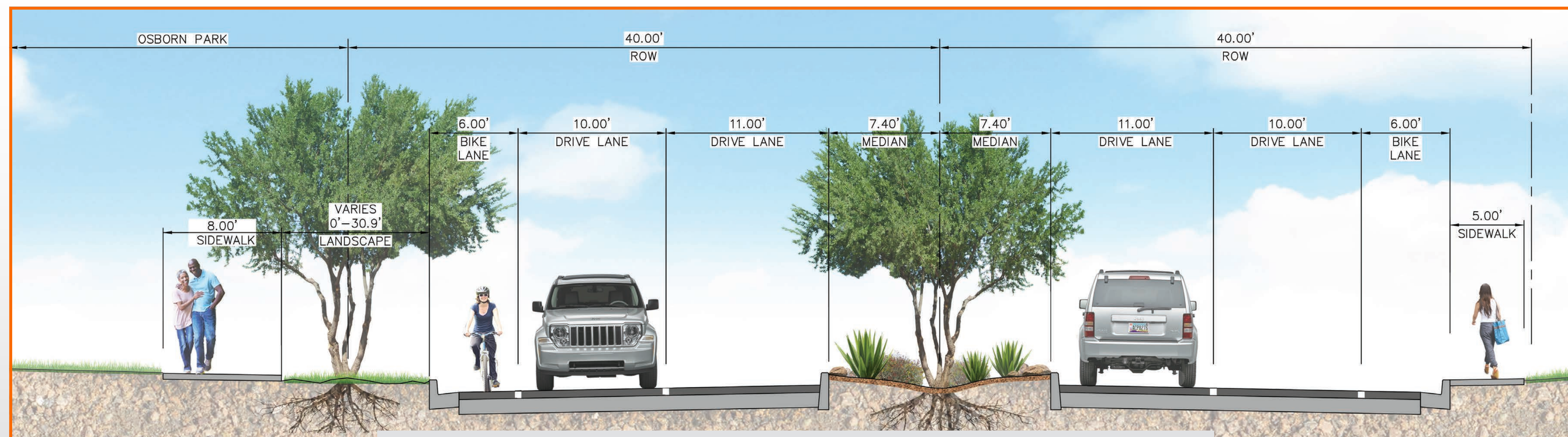
Osborn Road with Raised Median (Looking East)
