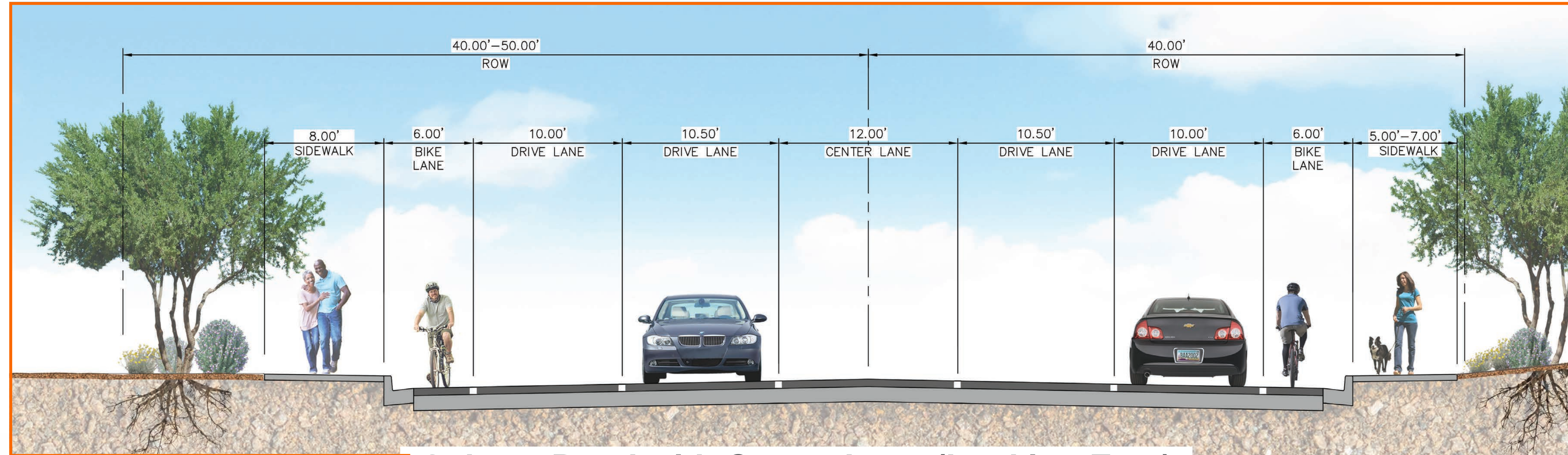
Osborn Road with Center Lane (Looking East)
