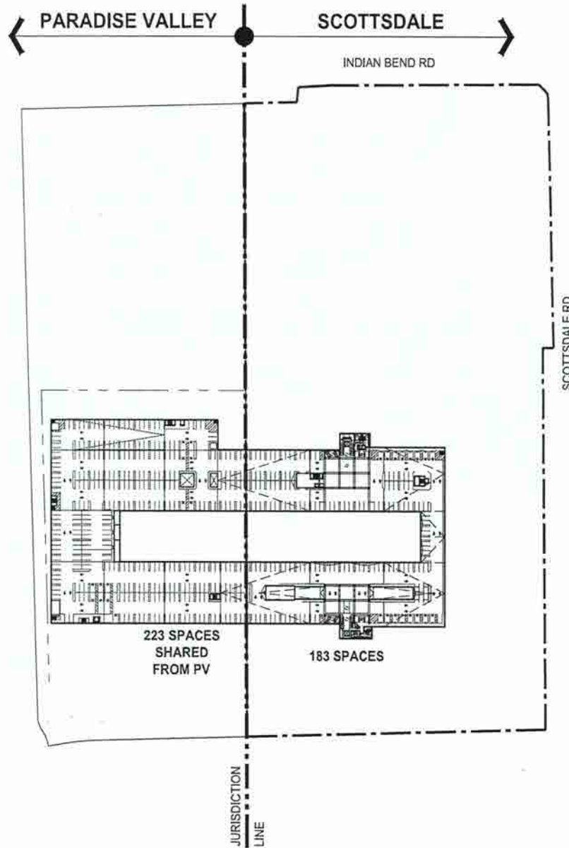
0 20' 40' NORTH 01 PARKING PLAN - B1 LEVEL SCALE: 1"=40' REF:
