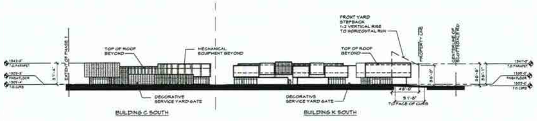
6750 NORTH OVERALL SOUTH ELEVATION 02 SCALE: 1/4"=1'-0" REF:
