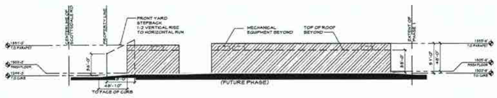
INDIAN BEND RD. OVERALL NORTH ELEVATION 01 SCALE: 1/4"=1'-0" REF:
