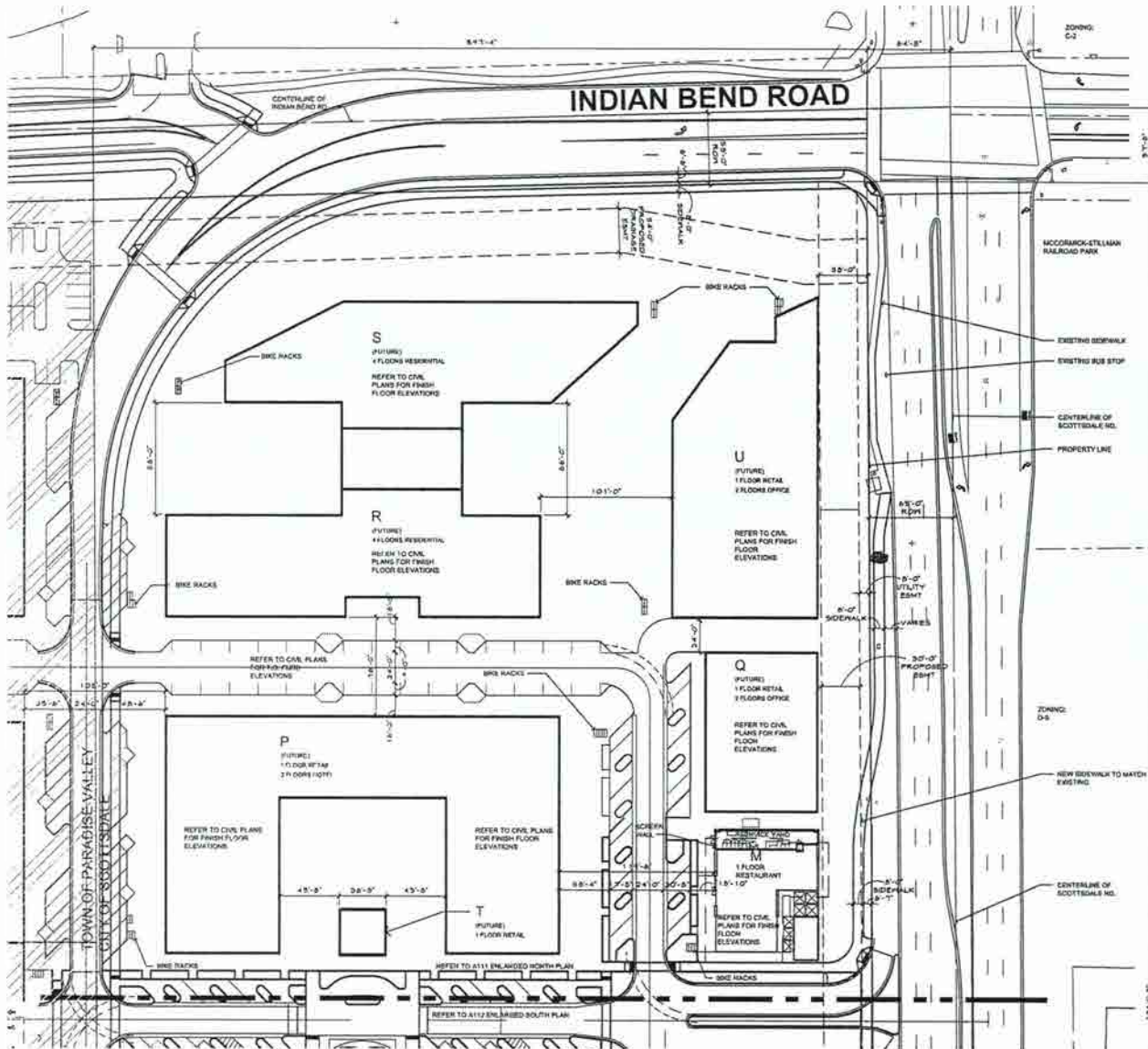
PHASE II 01 SITE PLAN - ENLARGED NORTH PLAN SCALE: 1"=40' REF:
