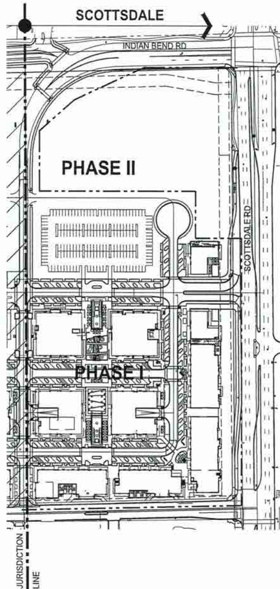
PHASE I PHASING PLAN SCALE: 1"=40' NORTH
