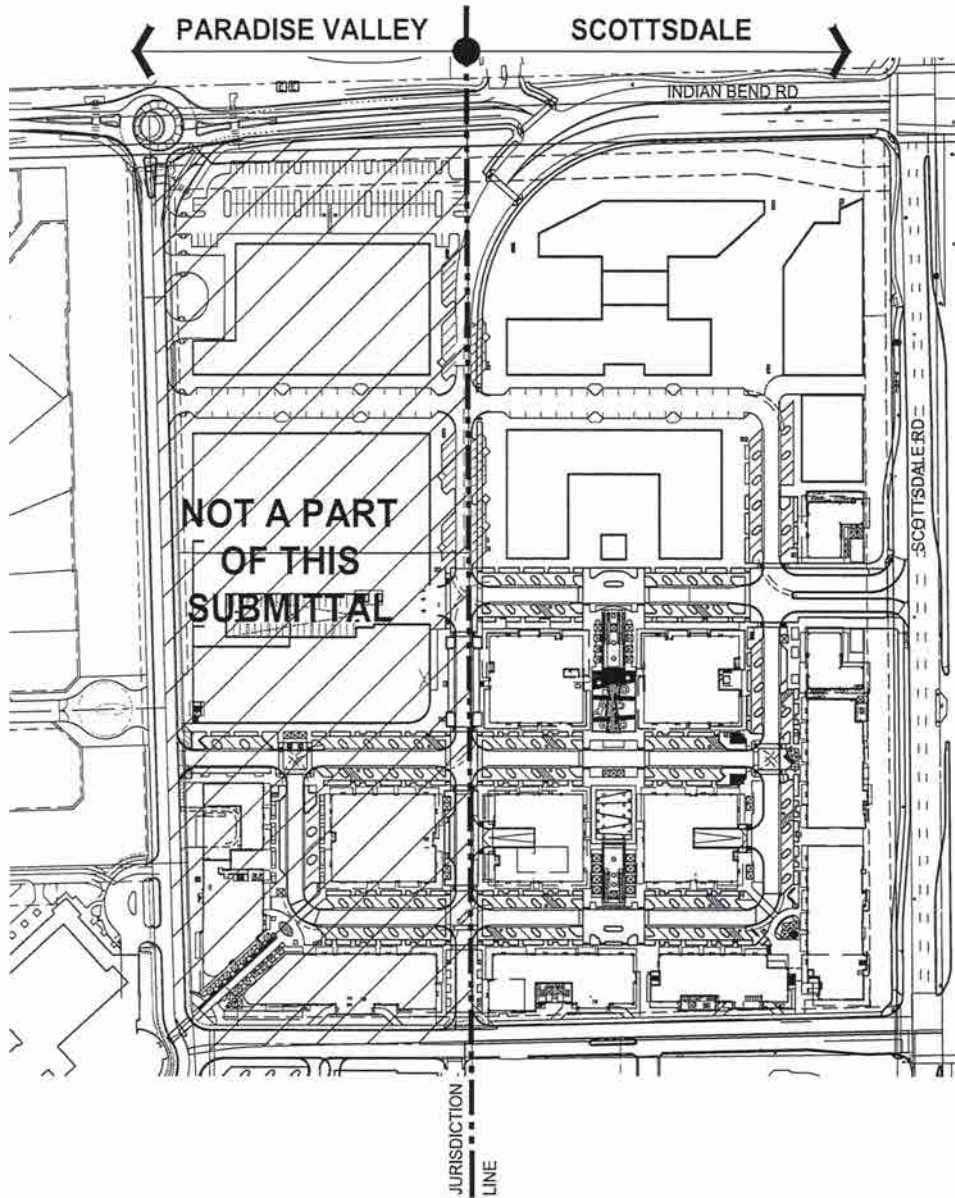
01 PARKING PLAN - SURFACE PARKING SCALE: 1"=40' REF.
