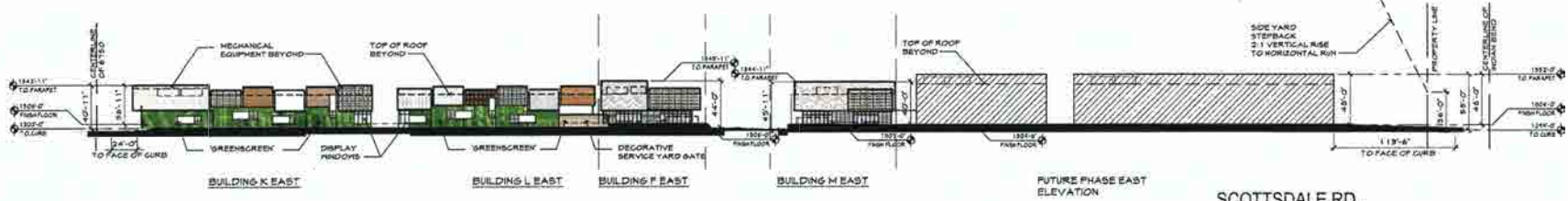
SCOTTSDALE RD. OVERALL EAST ELEVATION 03 SCALE: 1/4"=1'-0" REF:
