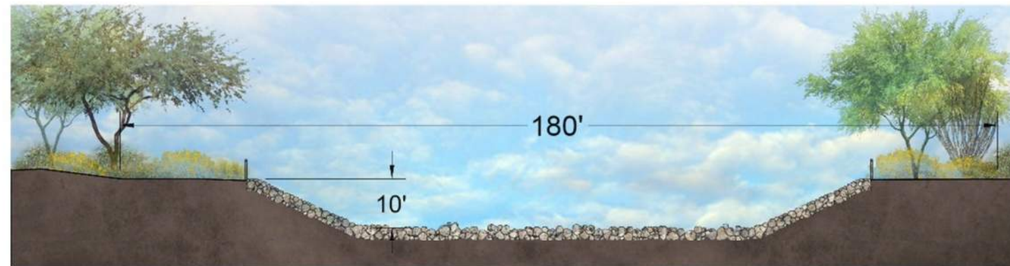
OPTION A: GROUTED ROCK CHANNEL LOWEST COST
