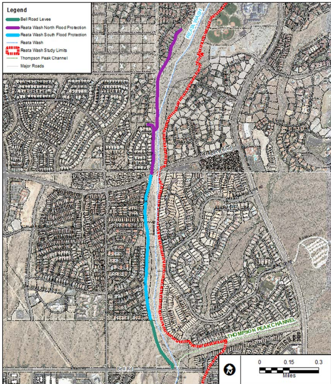
Figure 14.1 Reata Wash Potential Levees (Reach 4)
