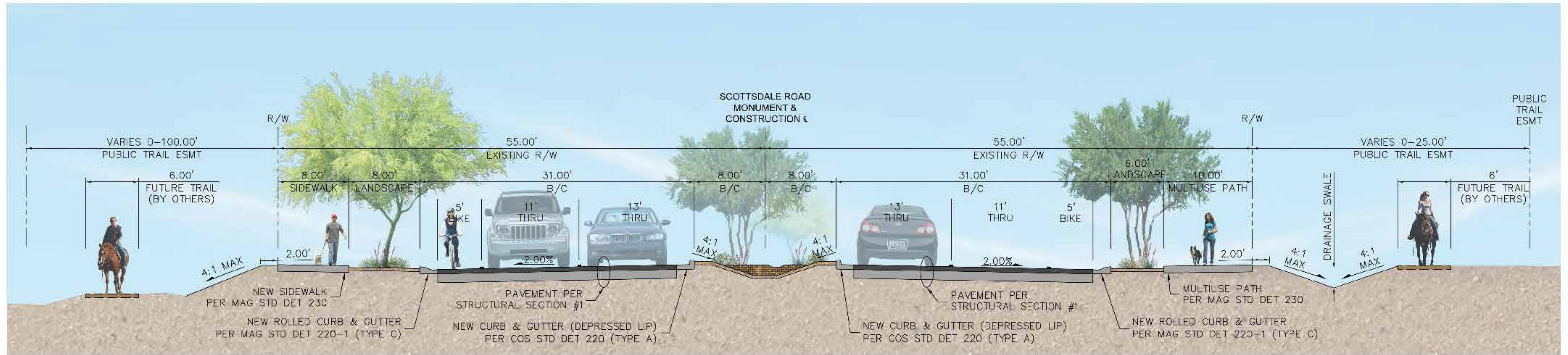
COMPLETE STREETS LANDSCAPE AND LID ELEMENTS "LOOKING NORTH" not to scale
