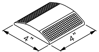
Pavement Marker (2-WAY REFLECTIVE BLUE) (ADOT TYPE BB) DETAIL "A"
