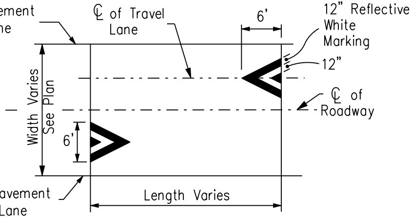
CHEVRON DETAIL
