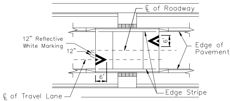
Chevron Detail
