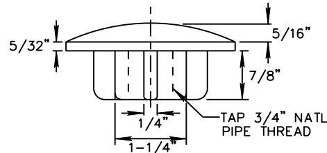
CAP DETAIL
