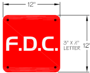
3" X 1/2" LETTERING (TYPICAL FOR ALL SIGNS)
